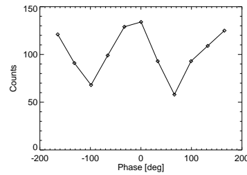
Fig. 4. Histogram of phase \phi(v_h - v_{ac}) obtained from IMAx data.
