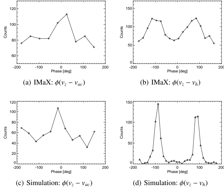
Fig. 3. (a) Histogram of phase \phi(v_z - v_{ac}) obtained from IMaX between the vertical velocity v_z in magnetic features and p-mode velocity in surroundings, v_{ac} . (b) Histogram of phase \phi(v_z - v_h) from IMaX, where v_h is the horizontal velocity of magnetic features. (c) Histogram of phase \phi(v_z - v_{ac}) from MHD simulations. (d) Histogram of phase \phi(v_z - v_h) from MHD simulations. Only those signals with a coherence larger than 0.8 outside the cone-of-influence of the wavelet diagram contribute to a histogram.
