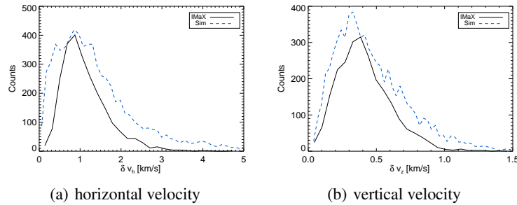
Fig. 2. (a) Histogram of amplitudes of the horizontal velocity. (b) Histogram of amplitudes of the vertical velocity.
