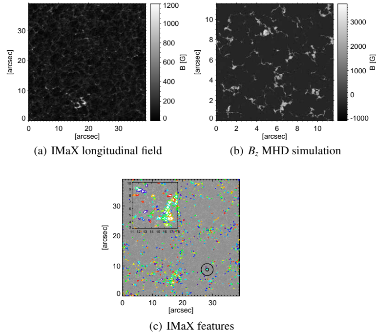
Fig. 1. (a) IMaX longitudinal field obtained from SIR inversions. (b) MHD simulation: longitudinal component of the magnetic field. (c) IMaX features tracking example. The two concentric circles bound the region surrounding the magnetic feature in which we consider the p-mode oscillations. Each color represents a label.
